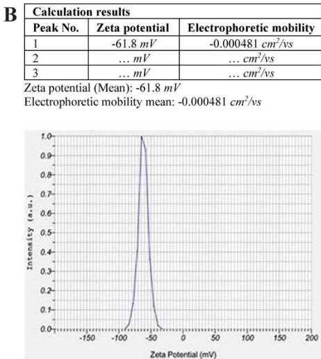
Figure 8. Zeta potential and electrostatic stability of nanoparticles extracted from AD-MSCs in the control group (A) and experimental group (B).
