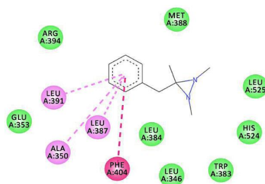
Figure 6. 2D view of the interaction between 1,2,3-Trimethyldiaziridine and amino acids in the binding site of estrogen receptor alpha.
