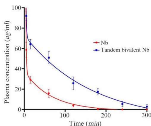
Figure 9. Plasma concentration monitoring of nanobody and tandem bivalent nanobody after injection in mice.
