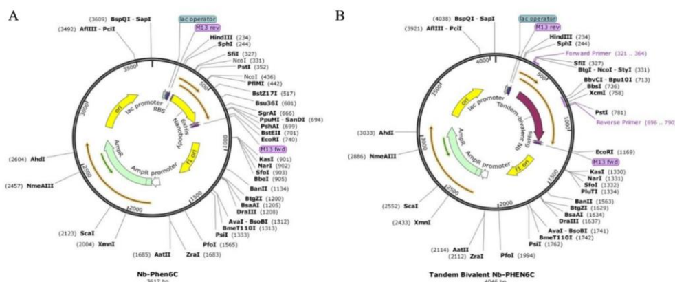
Figure 2. Schematic representation of (A) pHEN6-anti-VEGF 165 nanobody and (B) pHEN6c-VEGF 165 -bivalent plasmids.
