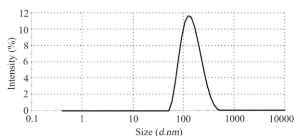
Figure 7. Hydrodynamic radius measuring tandem bivalent anti-VEGF 165 nanobody using dynamic light scattering.
