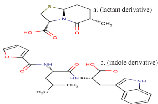
Figure 1. The structure of compound P (lactam derivative) and compound T (indole derivative).
