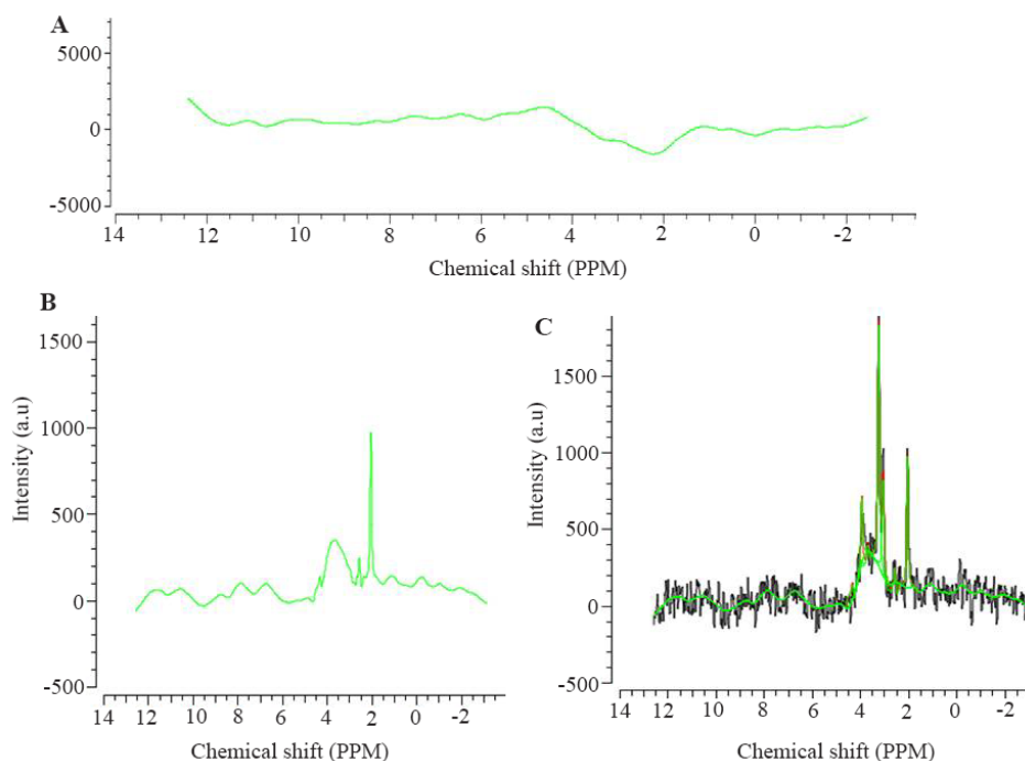
Figure 4. A) The baseline signal progenates from macromolecules. B) NAA signal selected as reference. C) Signal fitting is aimed at getting model signal from which concentration of metabolites can be calculated. The green curve shows the modeled signal.
