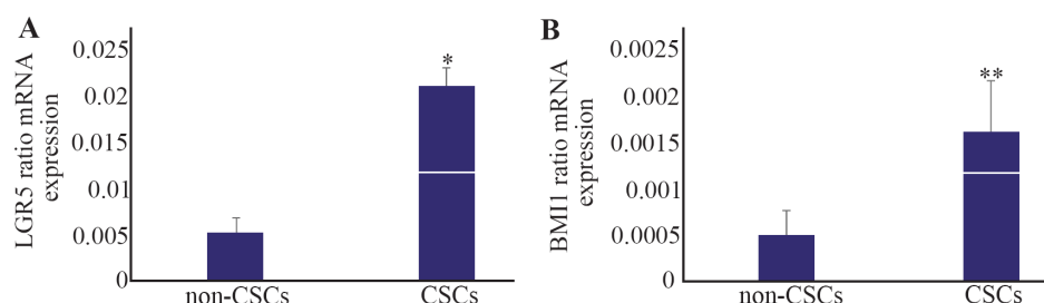
Figure 2. Relative mRNA expressions for leucine-rich repeat-containing G-protein-coupled receptor ( LGR5 ) and B cell-specific Moloney murine leukemia virus insertion site 1 ( BMI1 ) analyzed by real-time RT-PCR. A) LGR5 had high level of expression in the cancer stem-like cells (CSCs). B) BMI1 showed a similar pattern with higher rate of expression in the CSCs compared with the non-CSCs. * p \leq 0.001 and ** p \leq 0.03 vs. non-CSCs. Results are presented as mean \pm SD (n=14).
